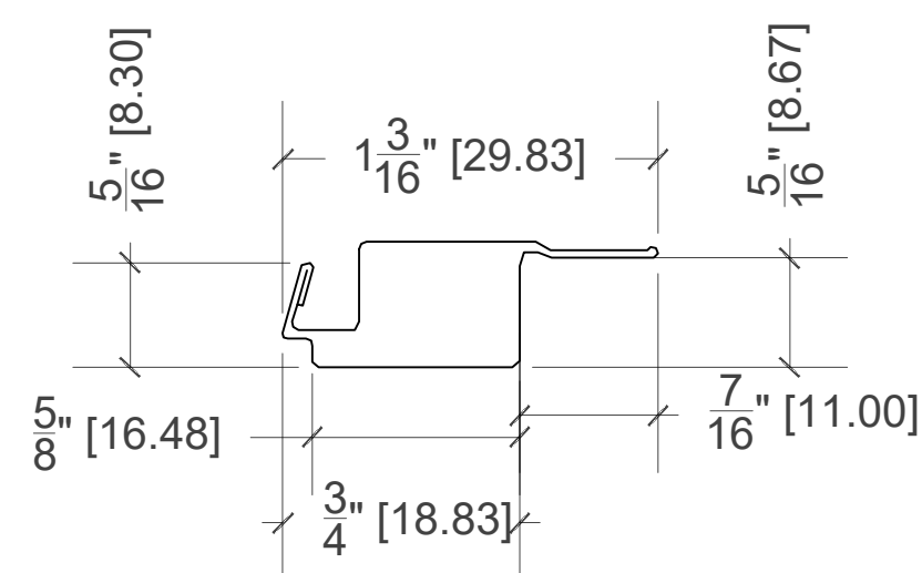
1 FIXED SCREEN FRAME PROFILE SCALE 18" = 1' - 0"
